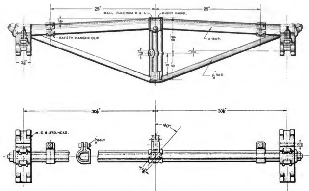
Figs. 4450-4451. Trussed U-Section Brake Beam. Simplex Railway Appliance Co.
